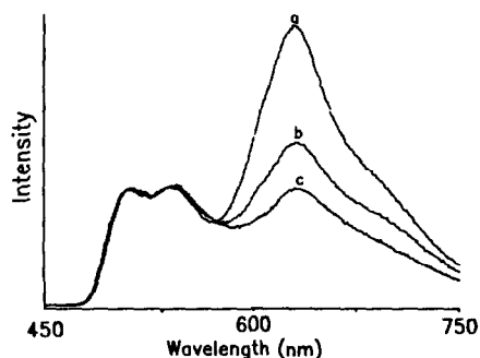
Figure 3. Emission spectrum of Pt(dmbpy)(ecda) in DMM glass at (a) 25 K, (b) 10 K, (c) 6 K.
