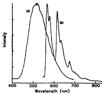
Figure 1. Emission spectrum of (a) \text{Pt}(\text{P}(\text{OPh})_3)_2(\text{mnt}) and (b) \text{Pt}(\text{P}(\text{O}-i\text{-Pr})_3)_2(\text{ecda}) at 77 K.
