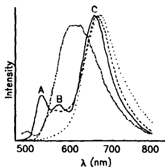
Figure 2. Emission spectrum of Pt(dpphen) in DMM glss at (---) 298 K, (···) 165 K, (-·-) 140 K and (—) 80 K.
